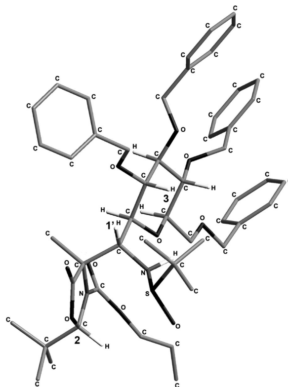
Figure 3. Spatial view of ( S S ,2 S ,4 R ,1' R )- 15 .
