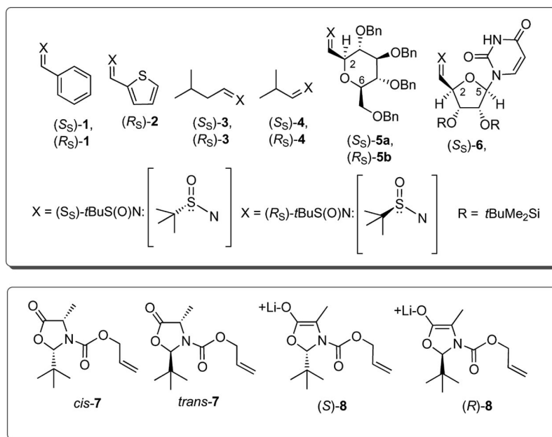
Figure 1. Oxazolidinones cis -7, trans -7 and their corresponding lithium enolates ( S )-8, ( R )-8, and ( S )- and ( R )-( N - tert -butylsulfinyl) aldimines 1–6.
