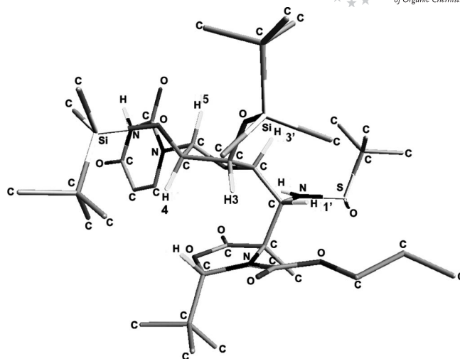
Figure 2. Spatial view of ( S S ,2 S ,4 R ,1' R )- 18 .
