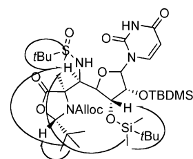
( S S ,2S,4R,1'R)- 18
